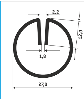
PROFILE LR 27 · 1.8
