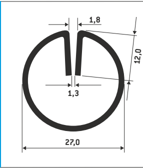
PROFILE LR 27 · 1.3
